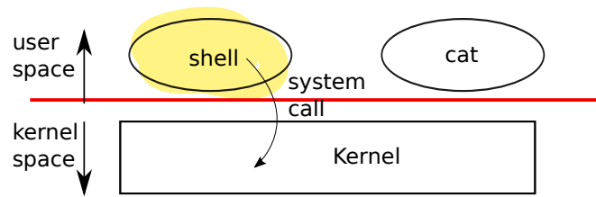
Figure 1.1: A kernel and two user processes.
