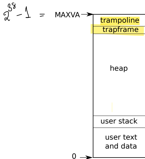
Figure 2.3: Layout of a process's virtual address space
